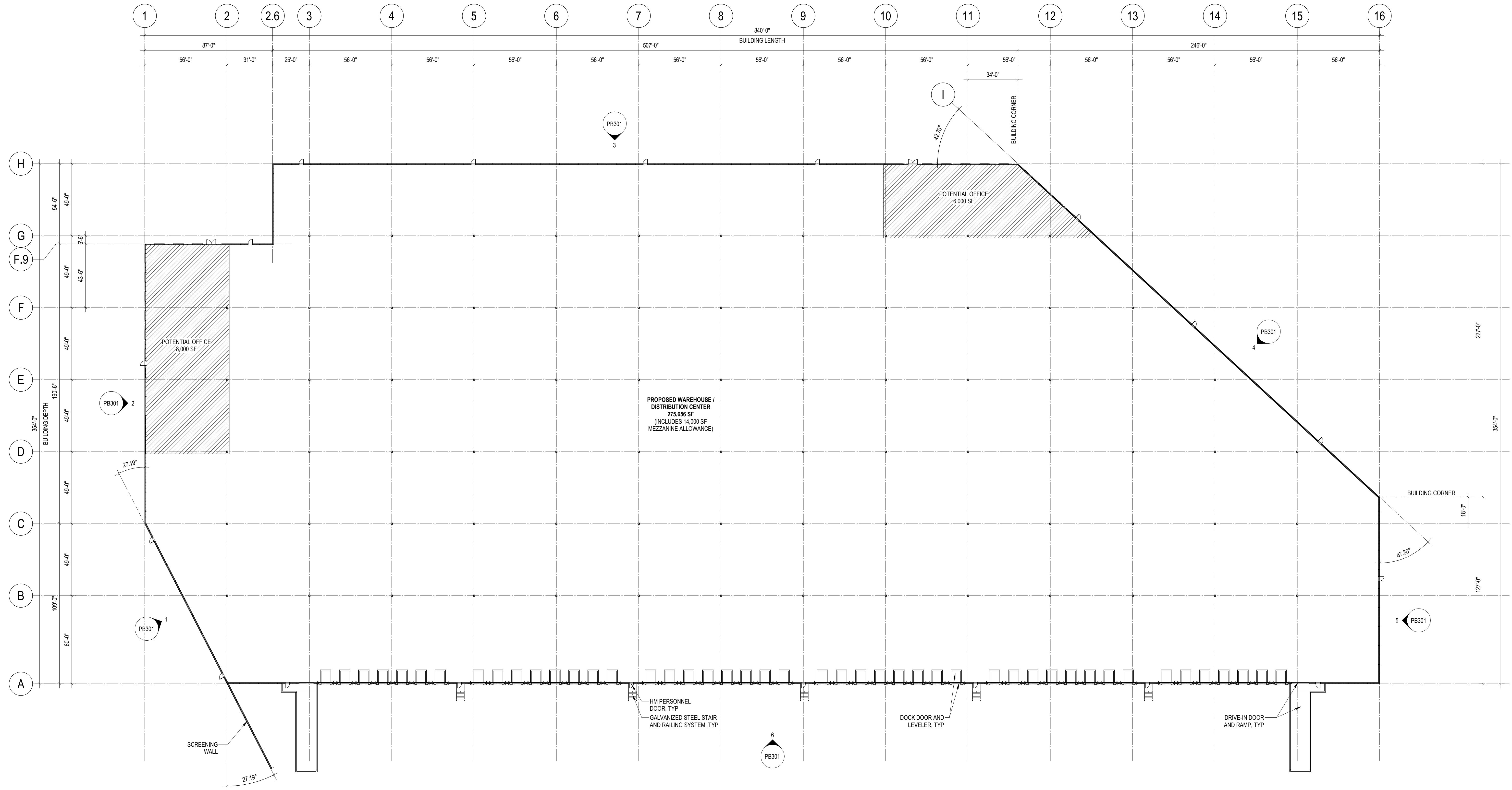
1 PB - OVERALL BUILDING PLAN PB101 1/32" = 1'-0"
